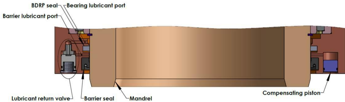
Figure 6 Using the BDRP as an RCD seal
