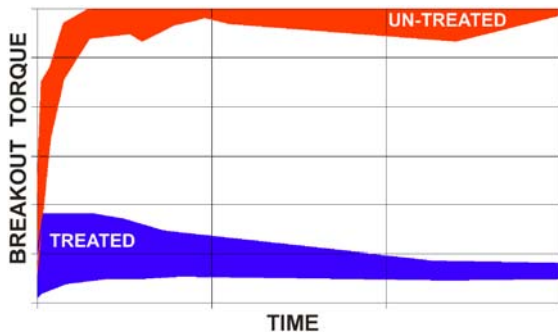
Figure 1 Breakout Torque Comparison
