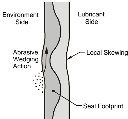
Figure 1 Skew-Induced Wear Mechanism
