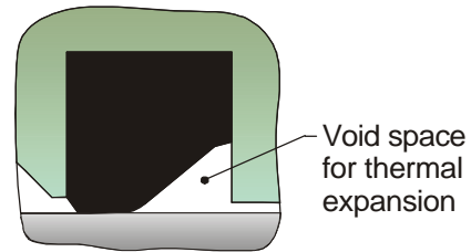
Figure 2 Axially Constrained Kalsi Seal
